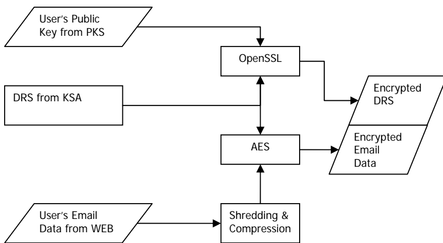
Figure 4: MyMail® dynamic encryption algorithm.
